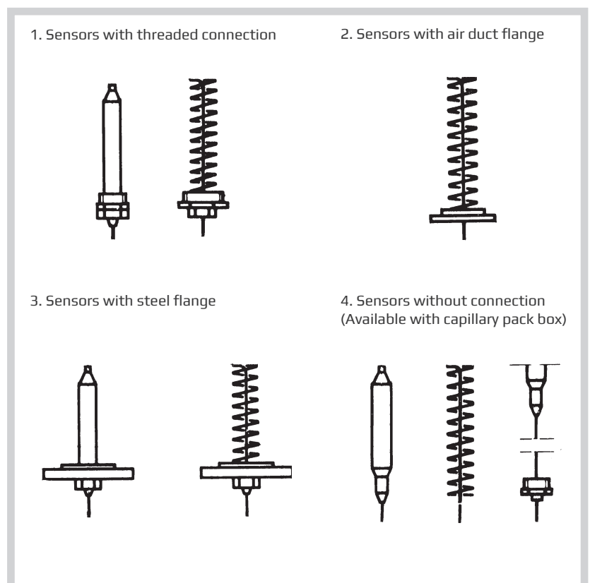
FIG. 4. SENSOR TYPES
